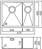
Volta 1.5 bowl Ref. VL53LBL £700 Overall size: 575/450 mm Bowl size: 340/400/190 mm Half bowl: 180/400/190 mm Cutout size: 555/430 mm (Inset) Minimum cabinet size: 600 mm Wastes included: 2 x 90 mm BSW & Plumbing Kit
