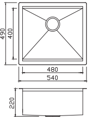
Stark Smart Single bowl Ref. SKS002 £449 Overall size: 540/490 mm Bowl size: 480/400/220 mm Cutout size: 520/470 mm (Inset) Minimum cabinet size: 600 mm Waste included: 90 mm BSW
