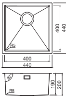
Volta Single bowl Ref. VL400S £300 Overall size: 440/440 mm Bowl size: 400/400/190 mm Cutout size: 420/420 mm (Inset) Minimum cabinet size: 500 mm Waste included: 90 mm BSW
