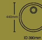
Arco Single bowl Ref. RB450B £128 Overall size: Ø440 mm Bowl size: Ø390/185 mm Cutout size: Ø416 mm Minimum cabinet size: 450 mm Waste included: 90 mm BSW
