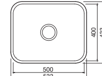
Tango Single bowl Ref. SP500 £260 Overall size: 533/433 mm Bowl size: 500/400/200 mm Minimum cabinet size: 600 mm
