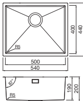
Volta Single bowl Ref. VL500S £335 Overall size: 540/440 mm Bowl size: 500/400/190 mm Cutout size: 520/420 mm (Inset) Minimum cabinet size: 600 mm Waste included: 90 mm BSW
