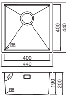
Volta Single bowl Ref. VL400BL £450 Overall size: 440/440 mm Bowl size: 400/400/190 mm Cutout size: 420/420 mm (Inset) Minimum cabinet size: 500 mm Waste included: 90 mm BSW
