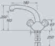
Venue Modern Mono Sink Mixer Ref. DCM104 Chrome £107 Min 0.1 bar pressure required Swivel Spout / Dual Flow Mounting hole size Ø 35mm WRAS Approved
