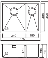
Volta 1.5 bowl Ref. VL53LS LH Main Bowl £535 Ref. VL53RS RH Main Bowl £535 Overall size: 575/450 mm Bowl size: 340/400/190 mm Half bowl: 180/400/190 mm Cutout size: 555/430 mm (Inset) Minimum cabinet size: 600 mm Wastes included: 2 x 90 mm BSW & Plumbing Kit
