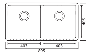
Buxton Double bowl Ref. TBU900 White £918 Installation: Apron Front Overall size: 895/465/229 mm Bowl sizes: 403/405/199 mm Overflow: Yes Tap-holes: No
