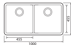
Cotswold Double bowl Ref. TCT1000 White £1374 Installation: Apron Front Overall size: 1000/535/220 mm Bowl sizes: 455/455/190 mm Overflow: Yes Tap-holes: No
