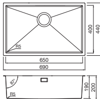
Volta Single bowl Ref. VL650S £390 Overall size: 690/440 mm Bowl size: 650/400/190 mm Cutout size: 670/420 mm (Inset) Minimum cabinet size: 800 mm Waste included: 90 mm BSW
