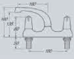
Venue Lever Deck Mounted Sink Mixer Ref. DLT105 Chrome £101 Min 0.1 bar pressure required Swivel Spout / Dual Flow Mounting hole size Ø 2 x 28mm WRAS Approved
