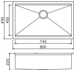
Stark Smart Single bowl Ref. SKS004 £639 Overall size: 800/490 mm Bowl size: 740/400/220 mm Cutout size: 780/470 mm (Inset) Minimum cabinet size: 1000 mm Waste included: 90 mm BSW
