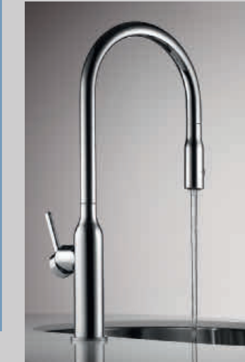
Ref. 10.261.002.000FL Sin single lever monobloc with swivel/pull-out spout Chrome £587 HP Min. 2.0 bar pressure required Flow rate at 3 bar: Neoperl® Cache 7ltrs per min NeedleSpray 6ltrs per min Hose pull-out length 50cm 360° swivel spout Mounting hole size Ø 35mm Lever installation on left or right side
