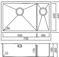
Volta 1.5 bowl Ref. VL68LS LH Main Bowl £605 Ref. VL68RS RH Main Bowl £605 Overall size: 735/450 mm Bowl size: 500/400/190 mm Half bowl: 180/400/190 mm Cutout size: 715/430 mm (Inset) Minimum cabinet size: 800 mm Wastes included: 2 x 90 mm BSW & Plumbing Kit
