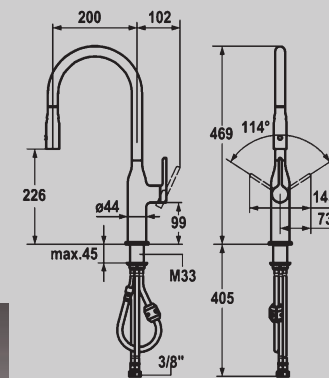
Ref. 10.261.002.000FL Sin single lever monobloc with swivel/pull-out spout Chrome £587 HP Min. 2.0 bar pressure required Flow rate at 3 bar: Neoperl® Cache 7ltrs per min NeedleSpray 6ltrs per min Hose pull-out length 50cm 360° swivel spout Mounting hole size Ø 35mm Lever installation on left or right side
