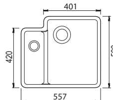
Nova 1.5 bowl Ref. NOV N150 £359 Right hand main bowl only Bowl size: 349/441/195 mm Half bowl: 163/361/160 mm Cutout size: Template Available Minimum cabinet size: 600 mm Standard waste kit included
