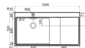
Xeron 105 Large bowl and drainer Ref. ML1F143A2 LHD £693 Ref. ML1F243A2 RHD £693 Overall size: 1000/520 mm Bowl size: 500/400/200 mm Cutout size: 982/502 mm Minimum cabinet size: 600 mm Waste included: 90 mm BSW
