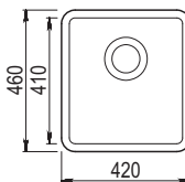
Nova Single bowl Ref. NOV N370 £299 Overall size: 420/460 mm Bowl size: 370/410/200 mm Cutout size: Template Available Minimum cabinet size: 450 mm Standard waste kit included
