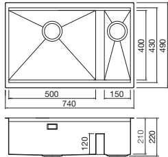
Stark Smart 1.5 bowl Ref. SKS006 £649 Overall size: 740/490 mm Bowl size: 500/400/220 mm Half Bowl: 150/400/220 mm Cutout size: 720/470 mm (Inset) Minimum cabinet size: 800 mm Wastes included: 2 x 90 mm BSW & Plumbing Kit
