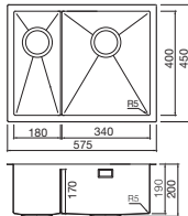
Volta 1.5 bowl Ref. VL53RBL £700 Overall size: 575/450 mm Bowl size: 340/400/190 mm Half bowl: 180/400/190 mm Cutout size: 555/430 mm (Inset) Minimum cabinet size: 600 mm Wastes included: 2 x 90 mm BSW & Plumbing Kit
