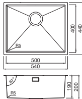
Volta Single bowl Ref. VL500BL £490 Overall size: 540/440 mm Bowl size: 500/400/190 mm Cutout size: 520/420 mm (Inset) Minimum cabinet size: 600 mm Waste included: 90 mm BSW
