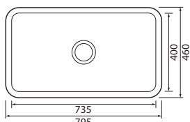
Essex Single bowl Ref. TES800 White £918 Installation: Apron Front Overall size: 795/460/254 mm Bowl size: 735/400/224 mm Overflow: Yes Tap-holes: No
