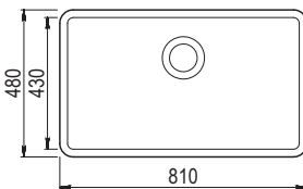
Nova Single bowl Ref. NOV N780 £439 Overall size: 810/480 mm Bowl size: 760/430/230 mm Cutout size: Template Available Minimum cabinet size: 1000 mm Standard waste kit included
